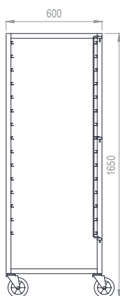
Vista Frontal
