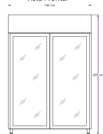
Vista Frontal
